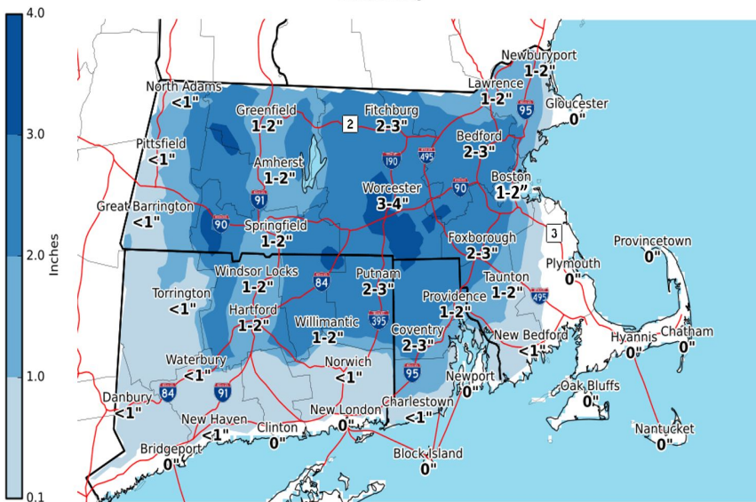
Expected Snowfall - Official NWS Forecast Valid: Friday
