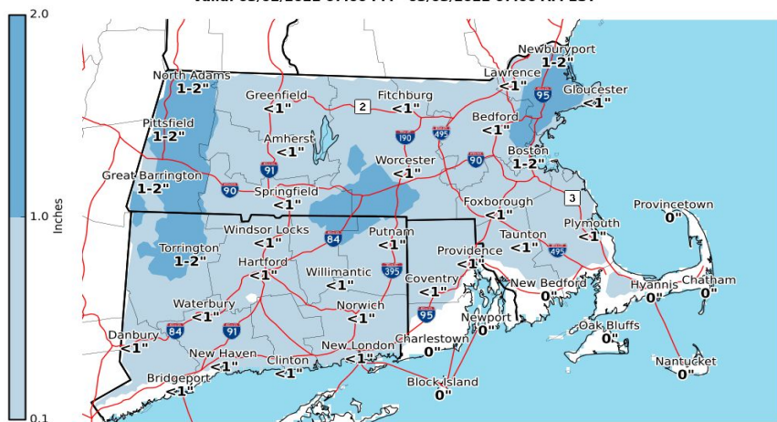
Expected Snowfall - Official NWS Forecast Valid: 03/02/2022 07:00 PM - 03/03/2022 07:00 AM EST
