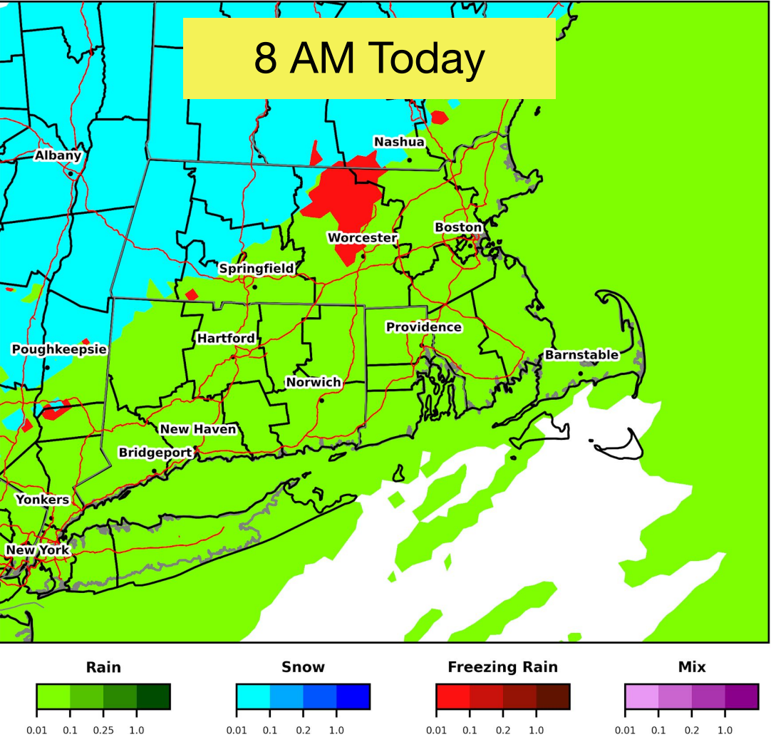
1-hr QPF/Dominant PType (in), HREF Model Guidance Valid January 23 2023 08 AM
